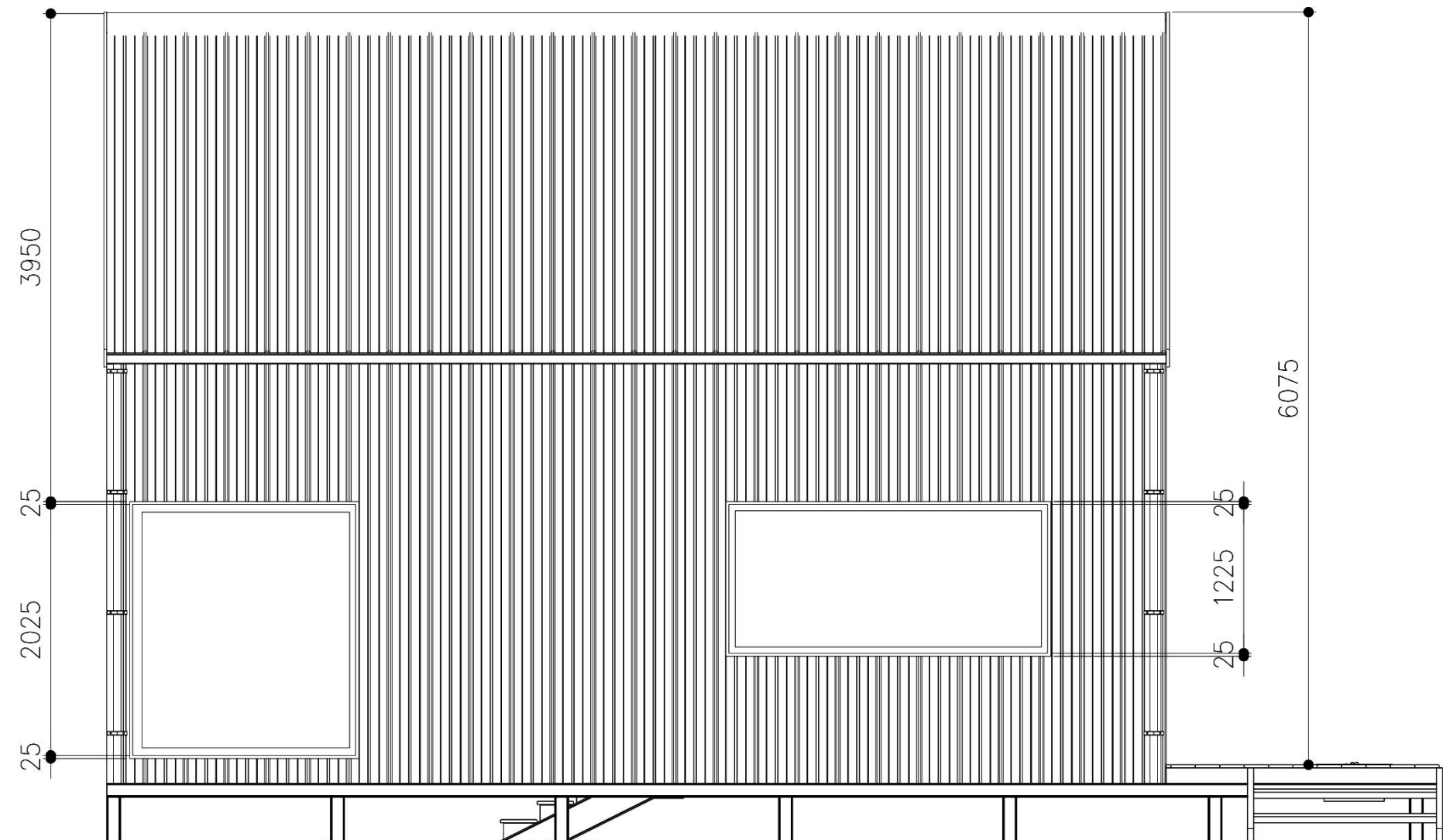
ELEVATION 03
