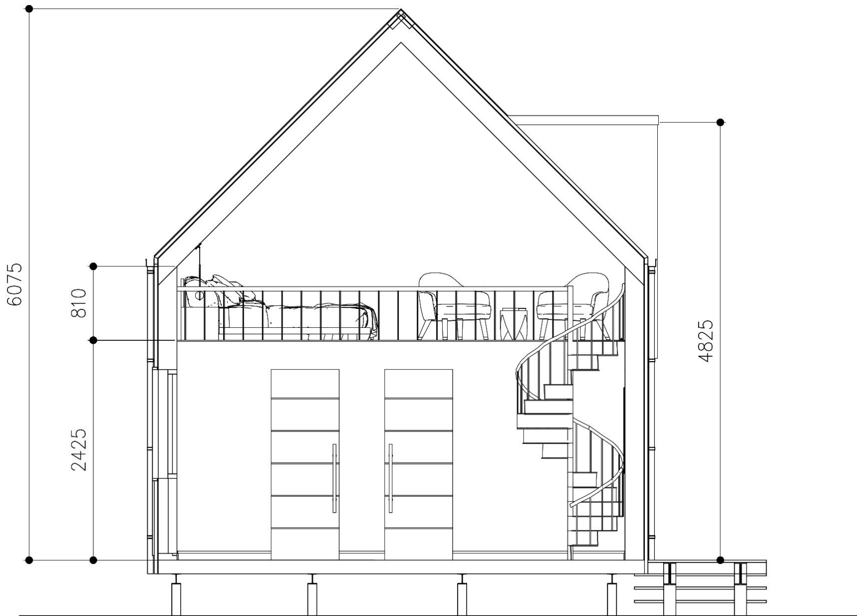
SECTION CUT
